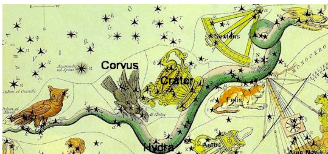
Urania's Mirror 1825
